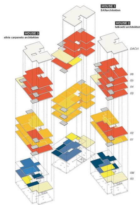
The division of program within one of the buildings. (Spreefeld Berlin / fatkoehl Architekten, n.d.)
